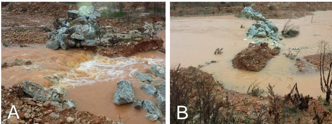
Figure 3.4: The overtopped rock check dams that separated the series of basins. Photo taken by author.
